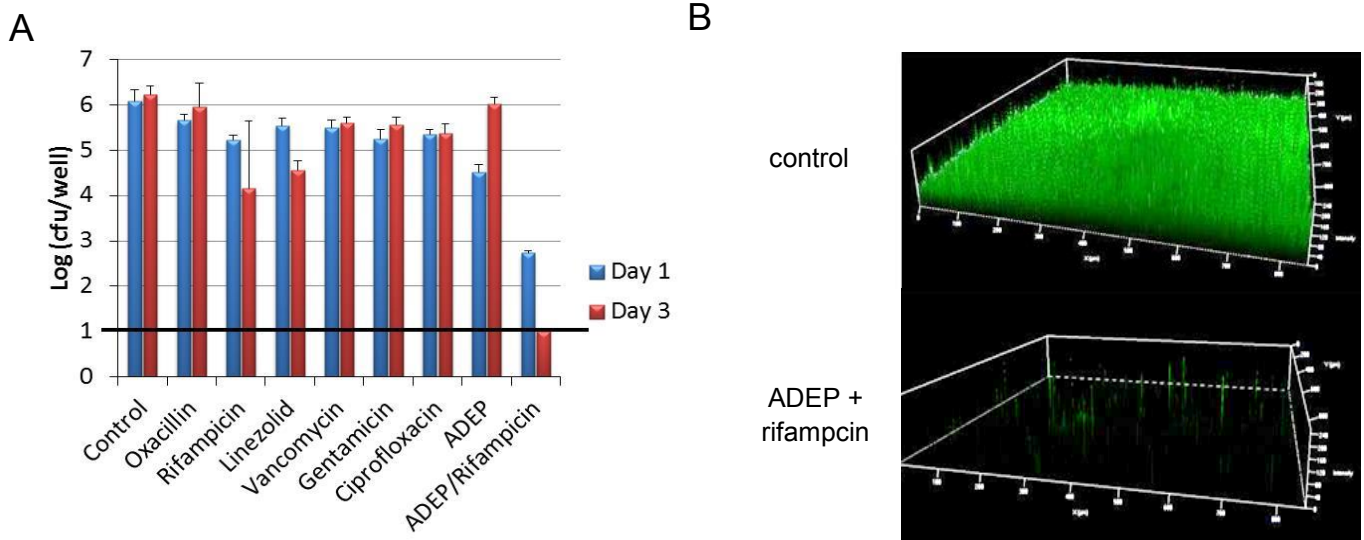
Figure 5. The effect of antibiotics on the survival of S. aureus biofilms. A) Biofilms were grown in 96 well plates and exposed to antibiotics at concentrations of 10x the MIC for 24 and 72 hours. B) Confocal microscopy live cell imaging of a control biofilms or one treated with the combination of ADEP and rifampicin at 1 and 10 x the MIC for 72 hours. S. aureus strain UAMS-1 was transformed with a GFP plasmid under the control of xylose inducible promoter. Biofilms were seeded and grown in an imaging flow cell for 24 hours. After drug exposure, the biofilms were washed with fresh medium containing xylose to induce GFP expression in live cells.
